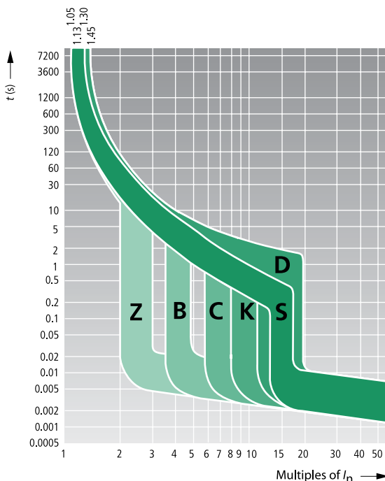
This graph shows trip-time versus over-current for all FAZ Supplementary Protectors.
